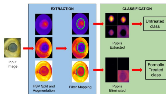
Figure 5. Framework of sssNet-SVM algorithm in classifying the C. chanos dataset.
